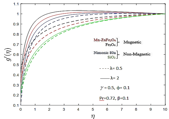
Figure 3: Magnetic stream function gradient, g'(\eta) for various reciprocal of magnetic Prandtl number ( \lambda )
