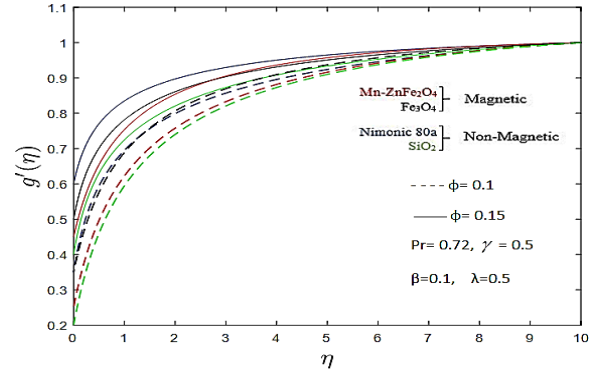
Figure 6: Magnetic stream function gradient, g'(\eta) for various nanoparticle solid volume fractions ( \phi )
