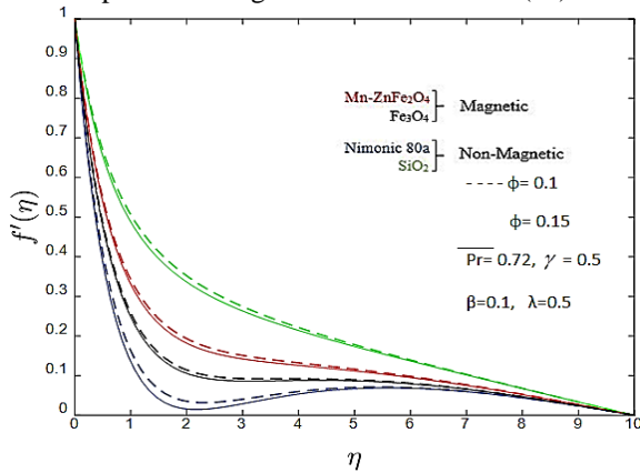
Figure 5: Velocity profiles, f'(\eta) for various nanoparticle solid volume fractions ( \phi )
