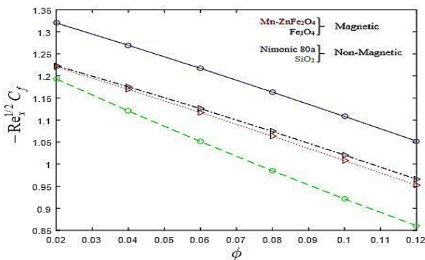
Figure 8: Surface shear stress distribution, f''(0) versus nanoparticle solid volume fraction ( \phi )
