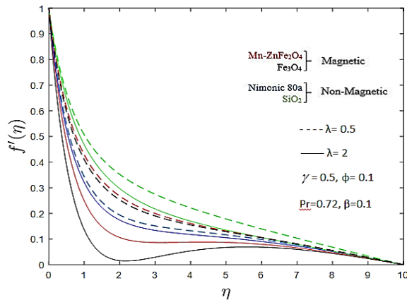
Figure 2: Velocity profiles, f'(\eta) for various reciprocal of magnetic Prandtl number ( \lambda )
