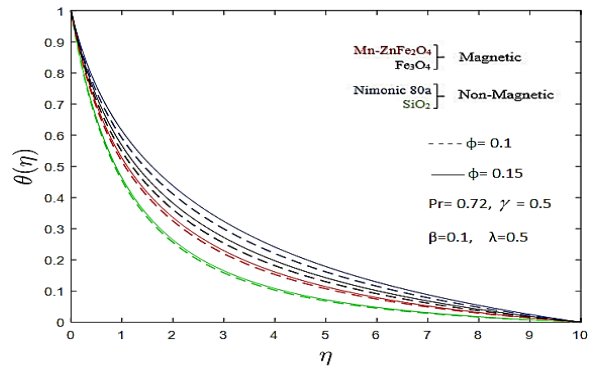
Figure 7: Temperature profiles, \theta(\eta) for various nanoparticle solid volume fractions ( \phi )
